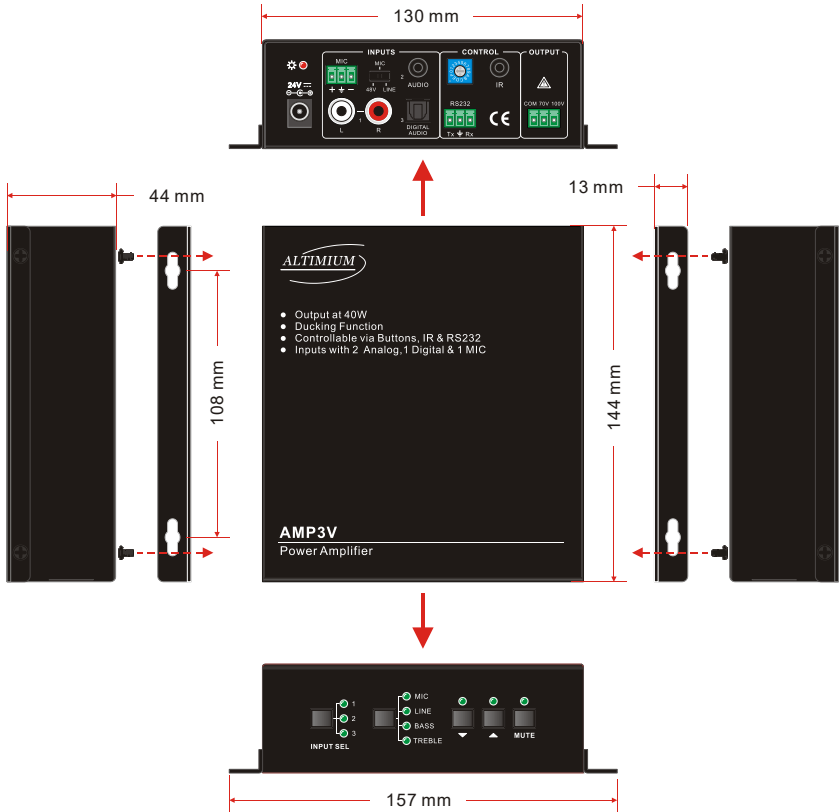
Figure 13 Panel Drawing
