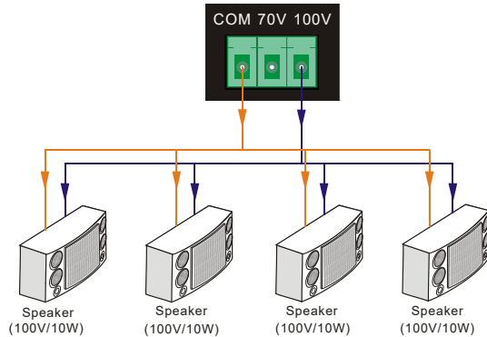
Figure 4 Audio Output Connection
